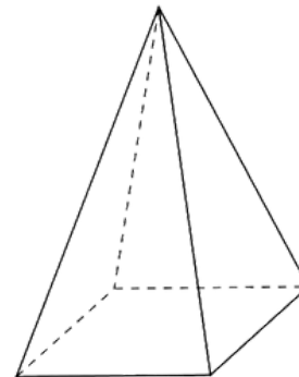
Pyramide
